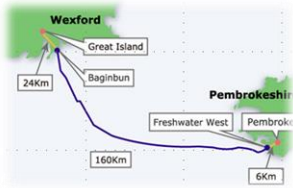
Ireland-UK Greenlink Interconnector
